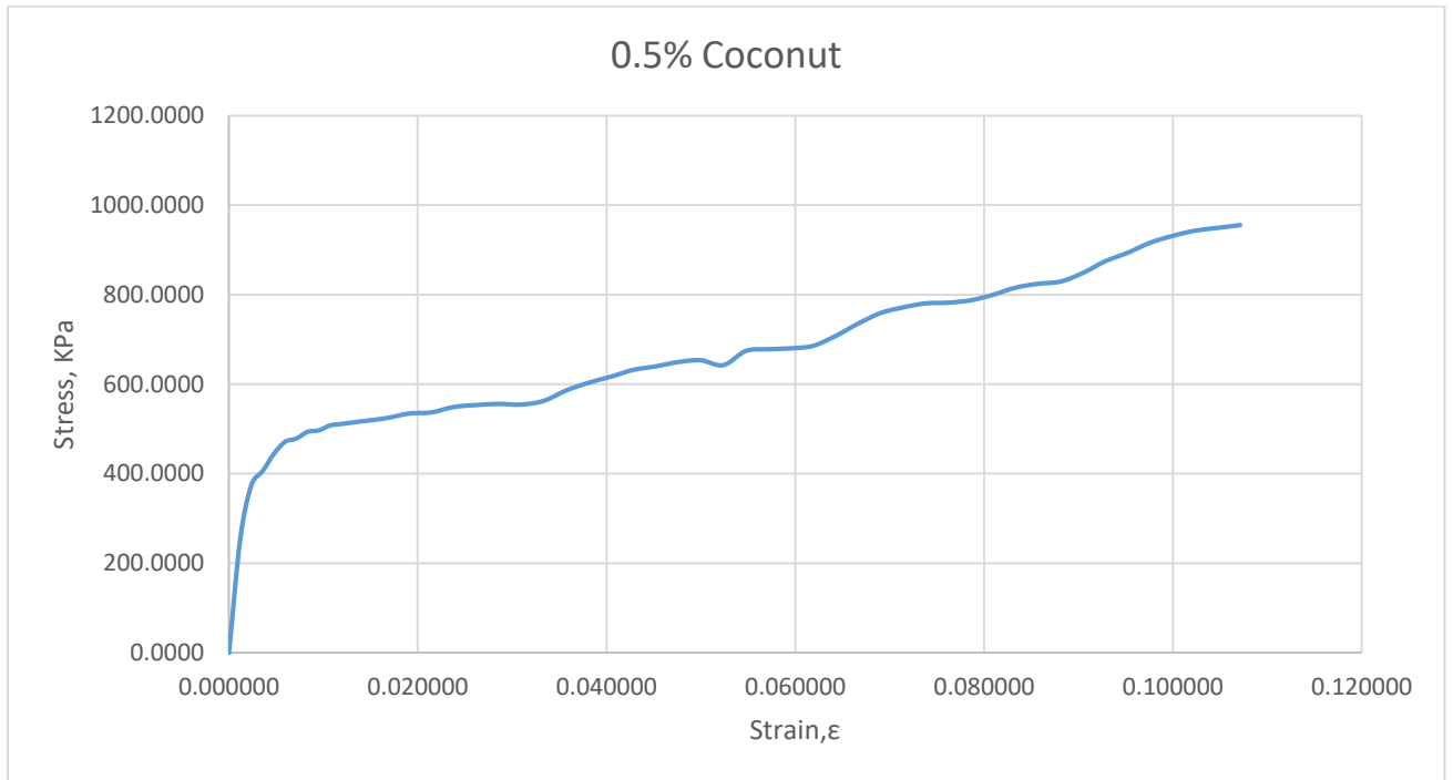
Figure 4.9 Stress vs Strain Curve of 0.5% Coconut fiber
