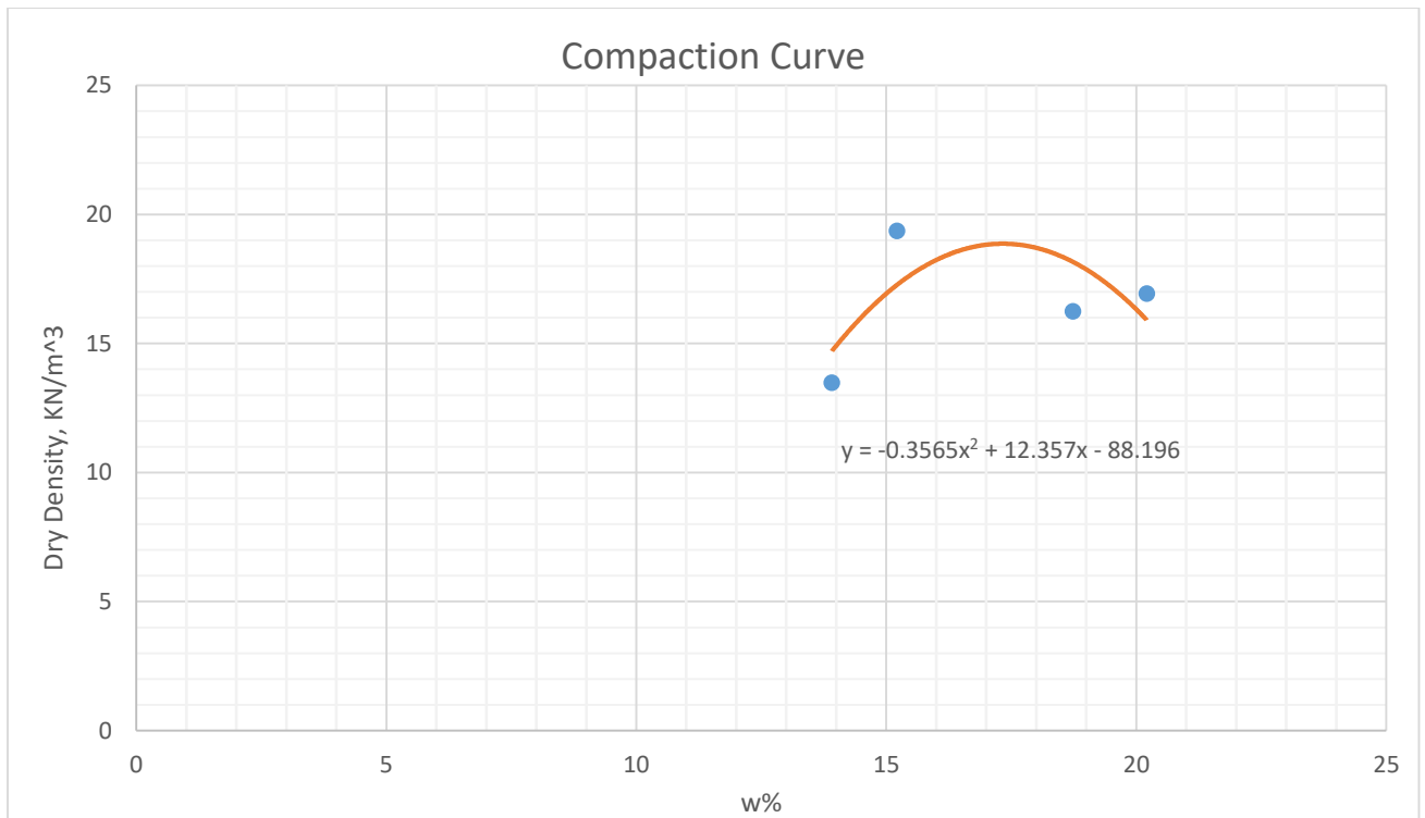
Figure 4.5 Compaction Curve
