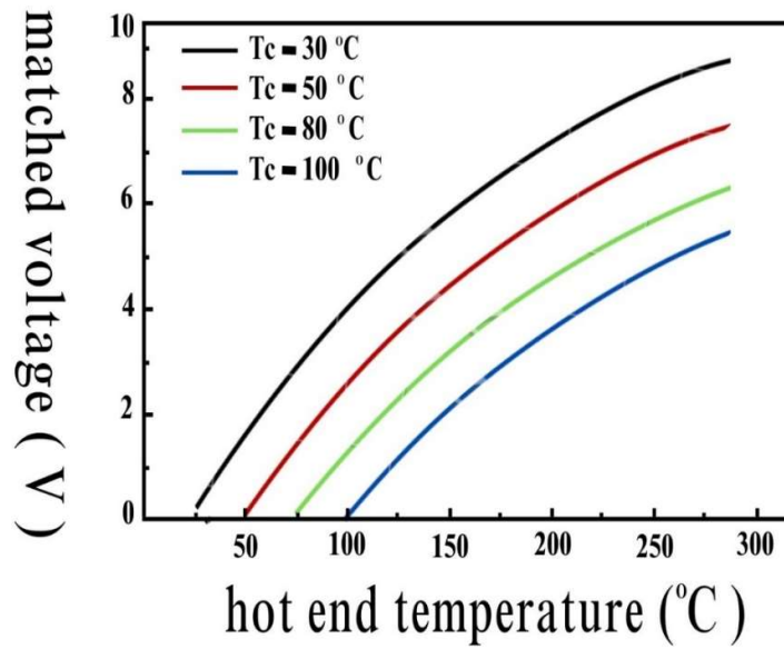
Figure 3: Matched voltage versus Hot end temperature
