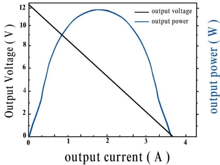
The chart output voltage and output power Vs output current under Th=300°C and Tc=30°C
