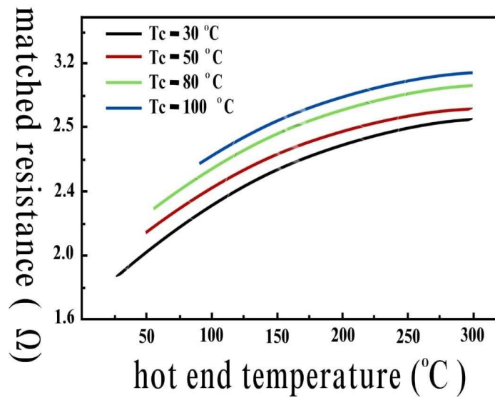
Figure 4: Matched resistance versus Hot end temperature
