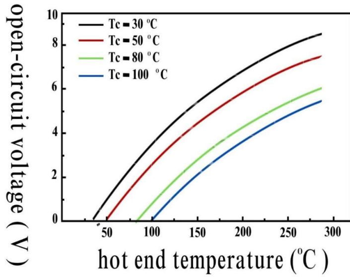
Figure 2: Thevenin voltage (open-circuit) versus Hot end temperature
