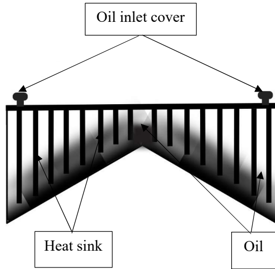
Figure 14: Heating oil tank of the Thermoelectric Generator.
