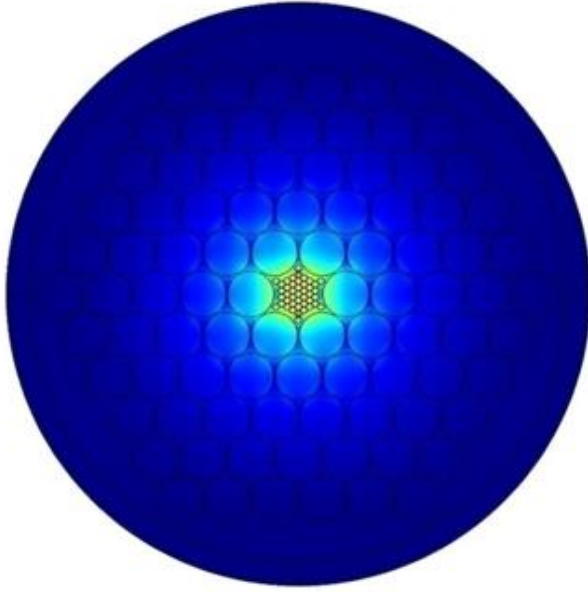
Fig 7.8: Hexagonal Cladding and Spider Core
