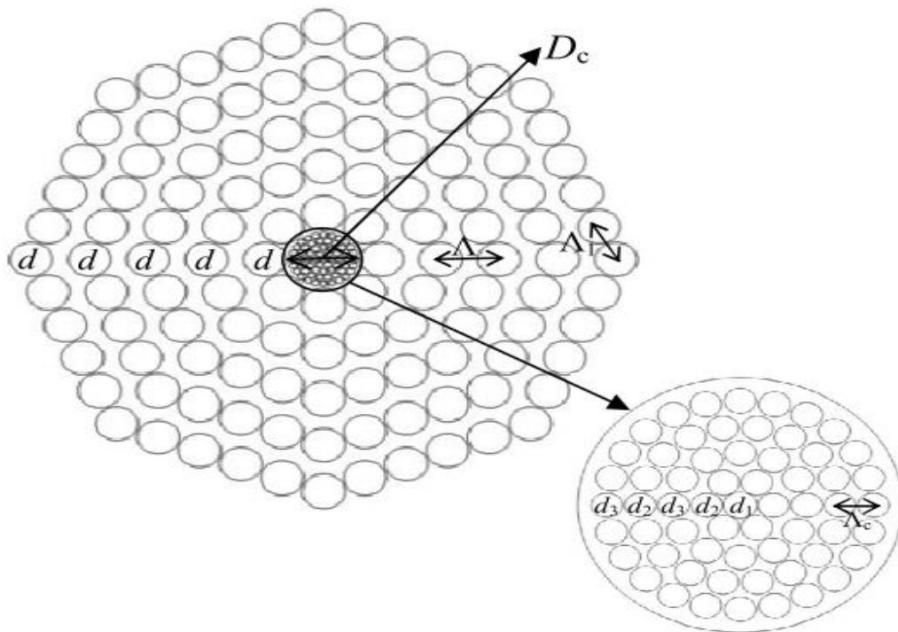
Fig 7.1: Transverse cross-section of five rings PC-OPCF
