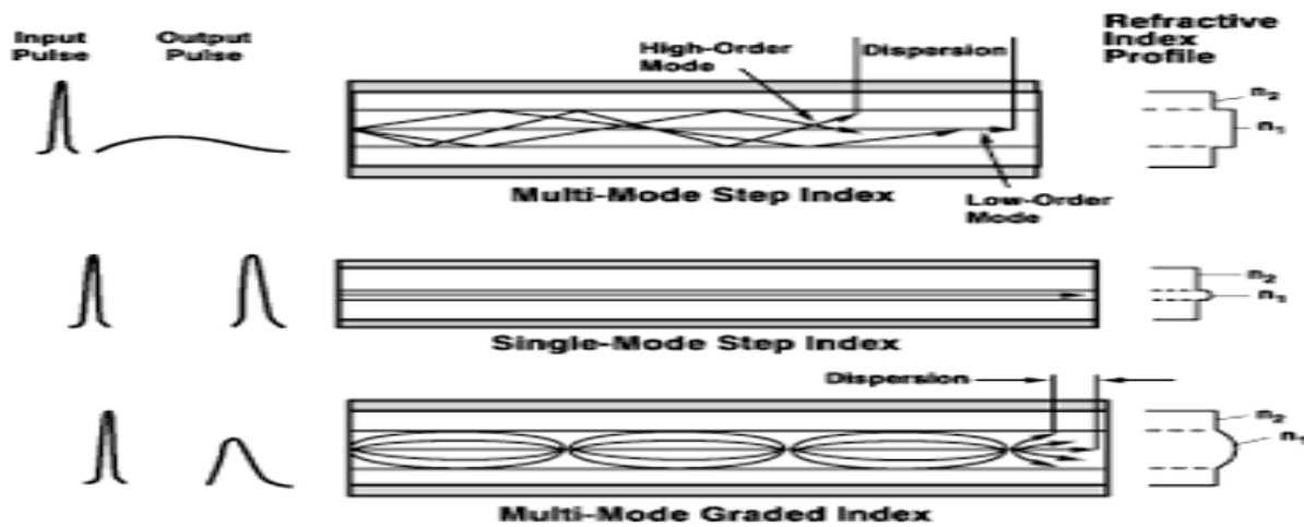
Fig 1.2: Optical Fiber Modes
