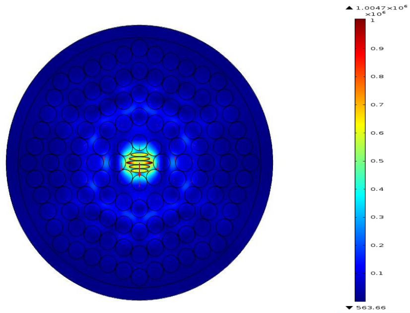
Fig 9.2: Power flow distribution of the proposed PCF
