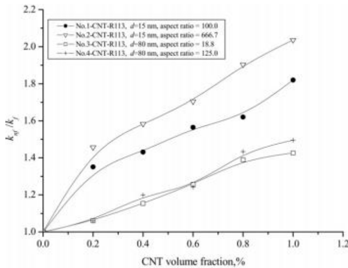
Fig. 1. k_{nf}/k_f of four kinds of CNT-R113 nanorefrigerants.
