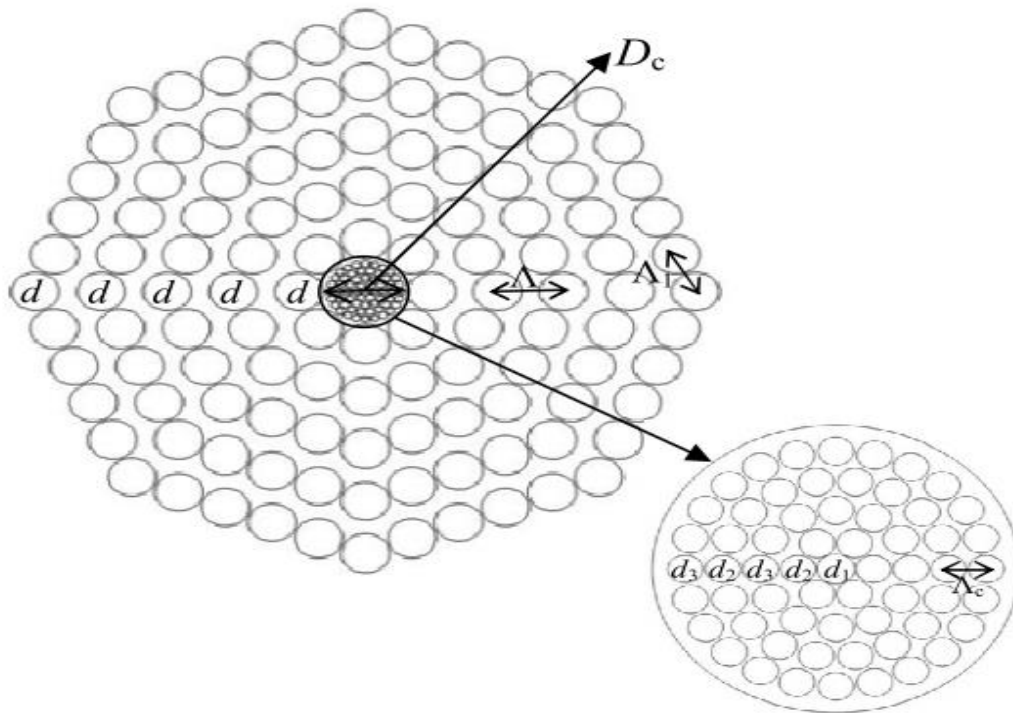
Fig 8.1: Transverse cross-section of five rings PC-OPCF
