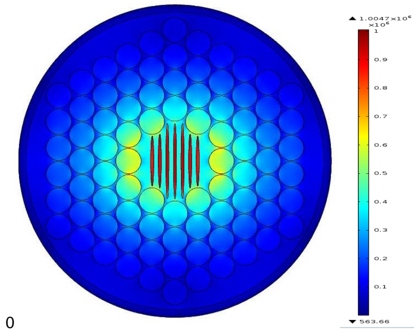
Fig 9.2: Power flow distribution of the proposed PCF
