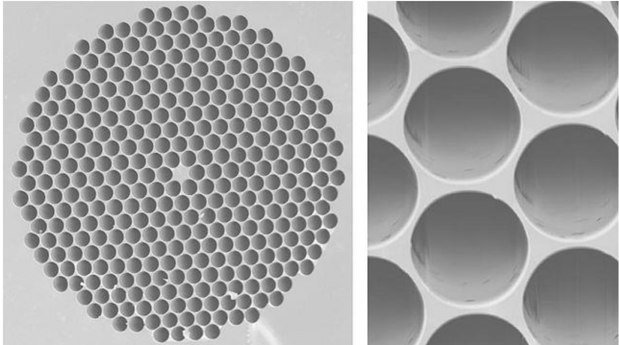
Fig 4.1: Photonic Crystal Fiber
