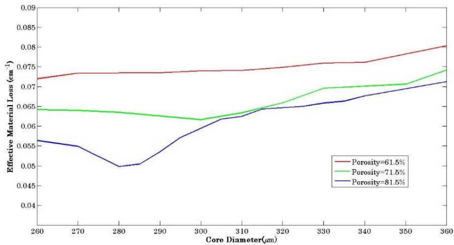
Fig 9.6: Effective material loss as a function of core diameter at different porosities
