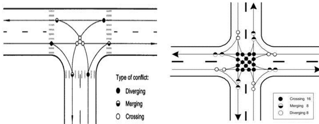
Figure 4-21: Tee legged & four-legged intersection
