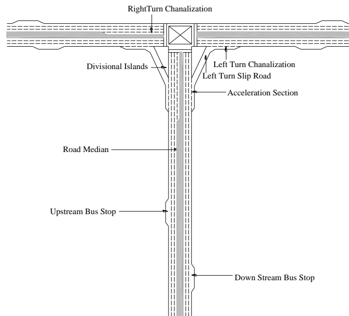
Figure 3-4: Typical tee or three legged intersection
