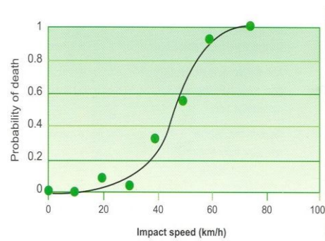
Figure 2-2: Death probability vs impact speed graph
